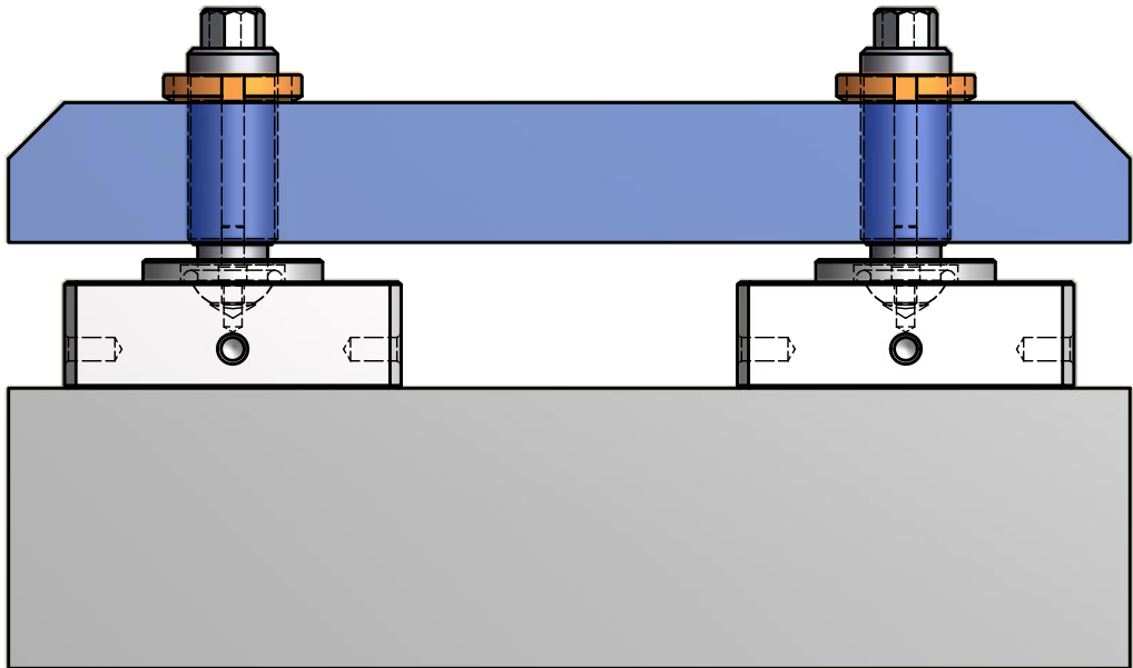
FRONT VIEW
