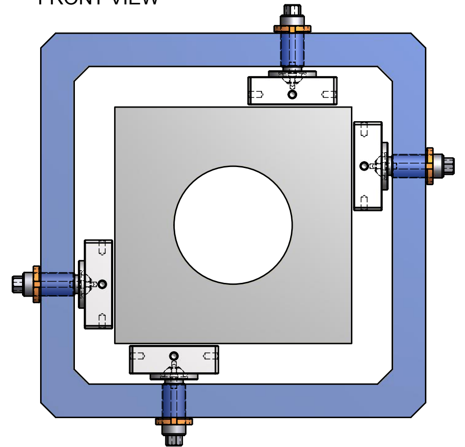
FRONT VIEW
